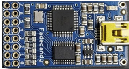
FadeCandy Board
